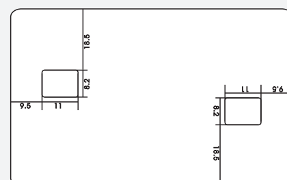
CONTACT IC CARD STRUCTURE
