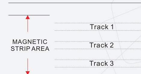
Structure of magnetic strip
